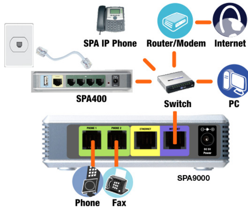
Linksys Voice System Overview
