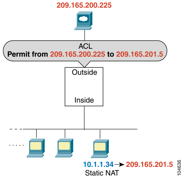
Figure 18-2 IP Addresses in Access Lists: NAT used for Destination Addresses
