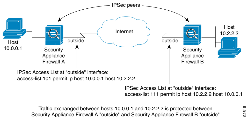
Figure 29-4 How Crypto Access Lists Apply to IPsec
