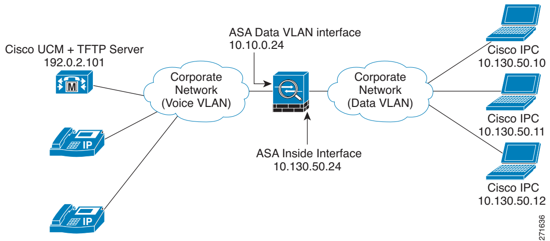
Figure 27-20 VLAN Transversal Between CIPC Softphones on the Data VLAN and Hard Phones on the Voice VLAN
