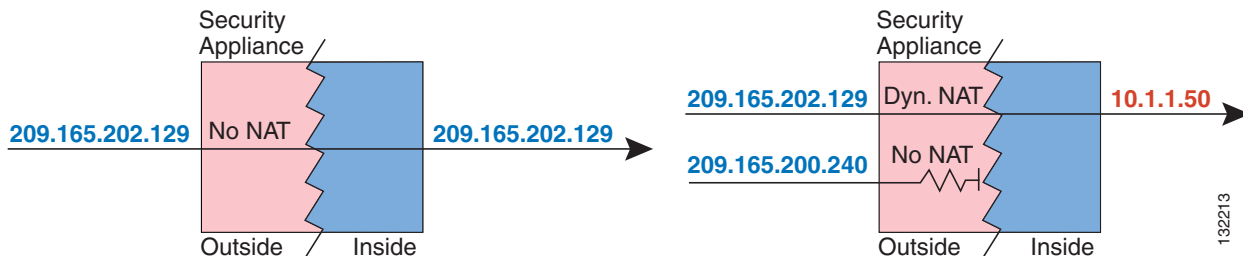
Figure 19-5 NAT Control and Inbound Traffic
