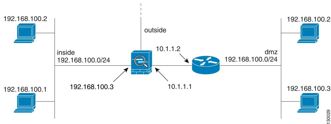
Figure 19-28 Using Outside NAT with Overlapping Networks
