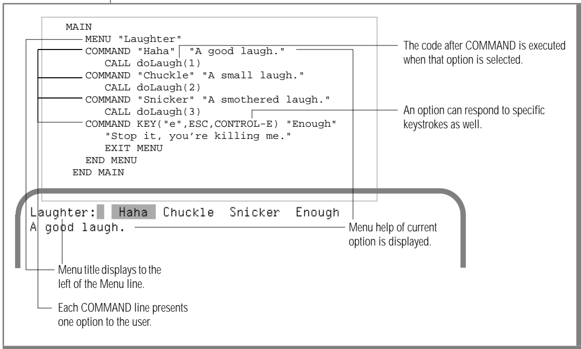
Figure 7-3 Menu-Driven Program
