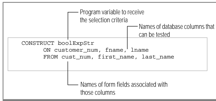
Figure 7-8 CONSTRUCT Statement
