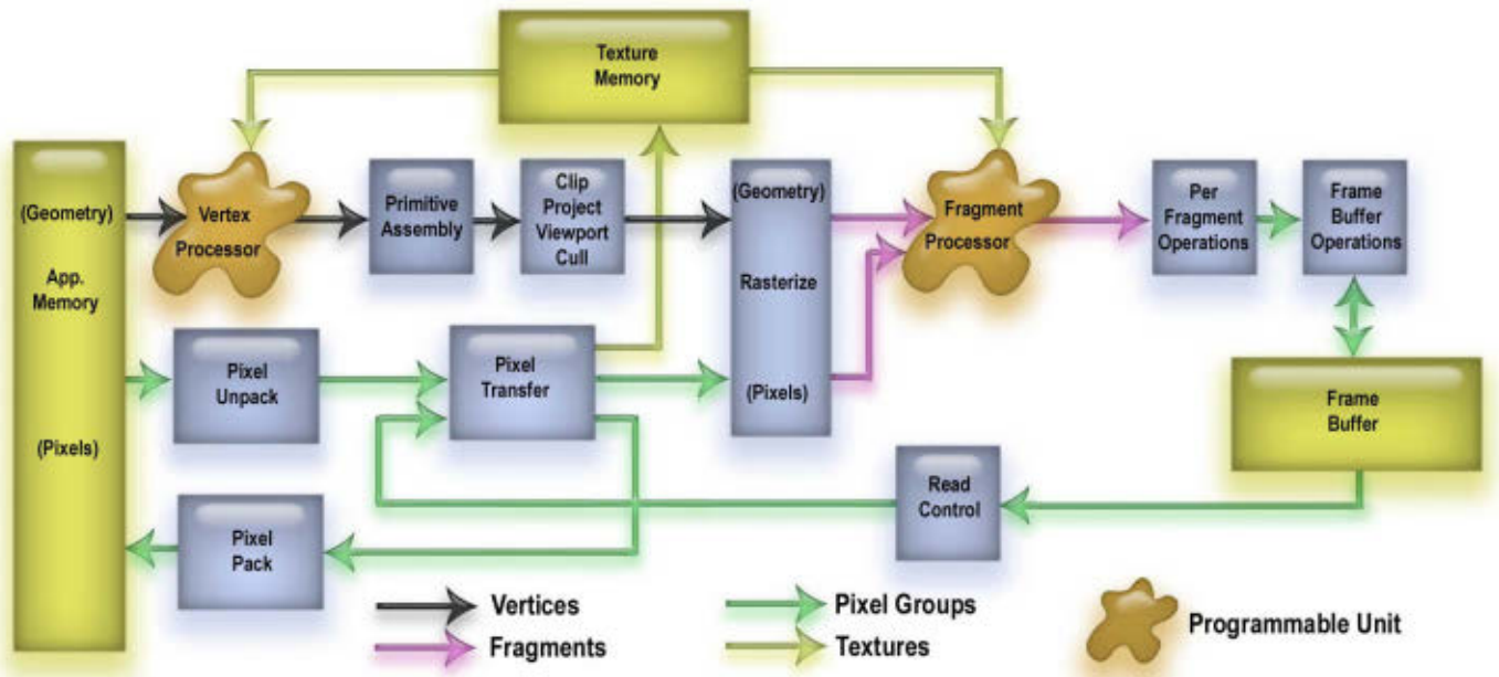
Figure 2. OpenGL Architecture
