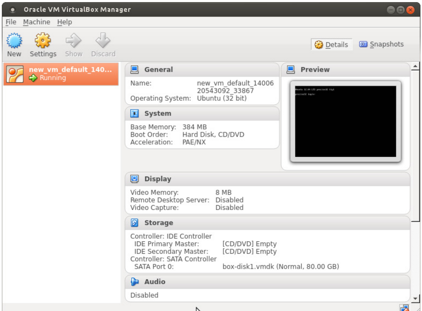
Figure 1. VirtualBox Screenshot
